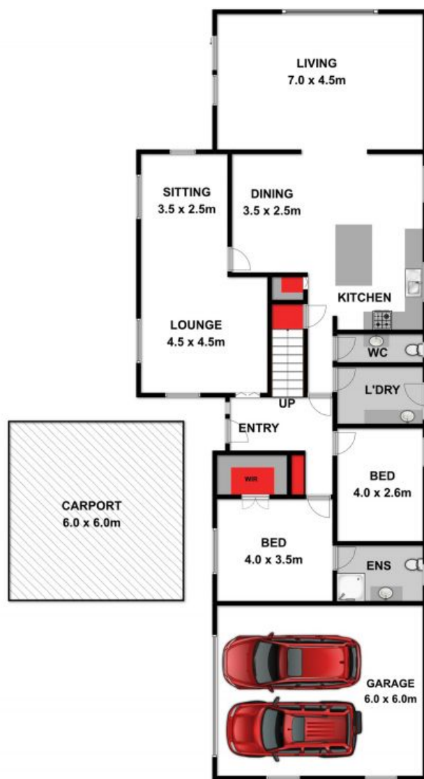
GROUND LEVEL
