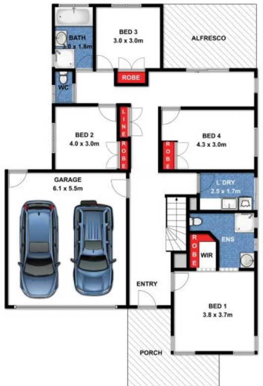
Ground Level
