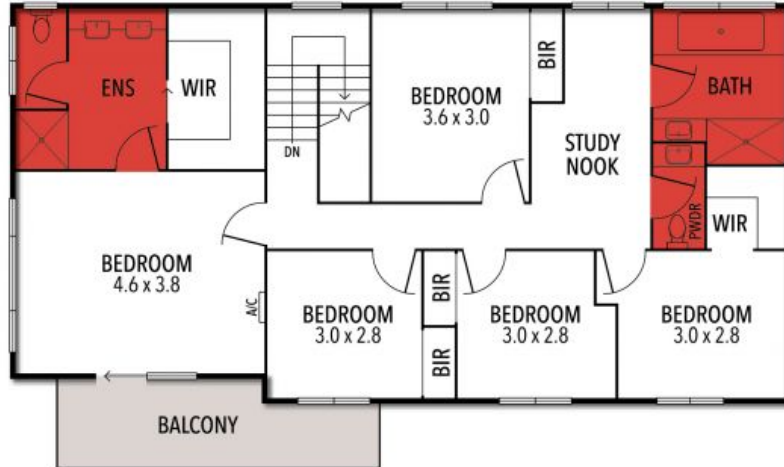
FIRST FLOOR
