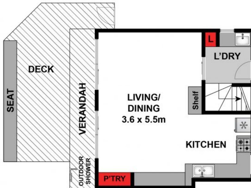
GROUND LEVEL
